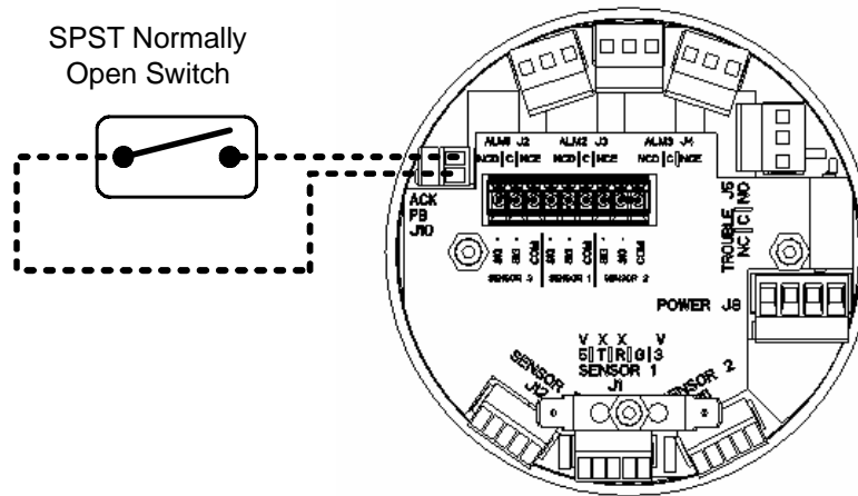
Figure 2-3. Push-button Wiring
